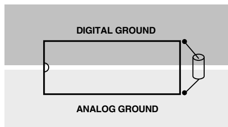
Figure 32. Ground Plane Layout
