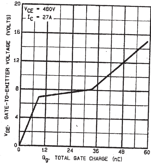
Fig. 8 - Typical Gate Charge vs. Gate-to-Emitter Voltage
