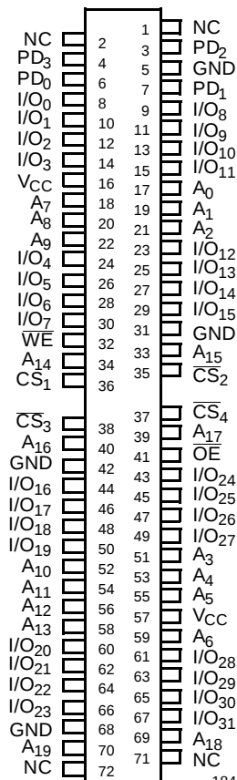
72-Pin SIMM Top View
