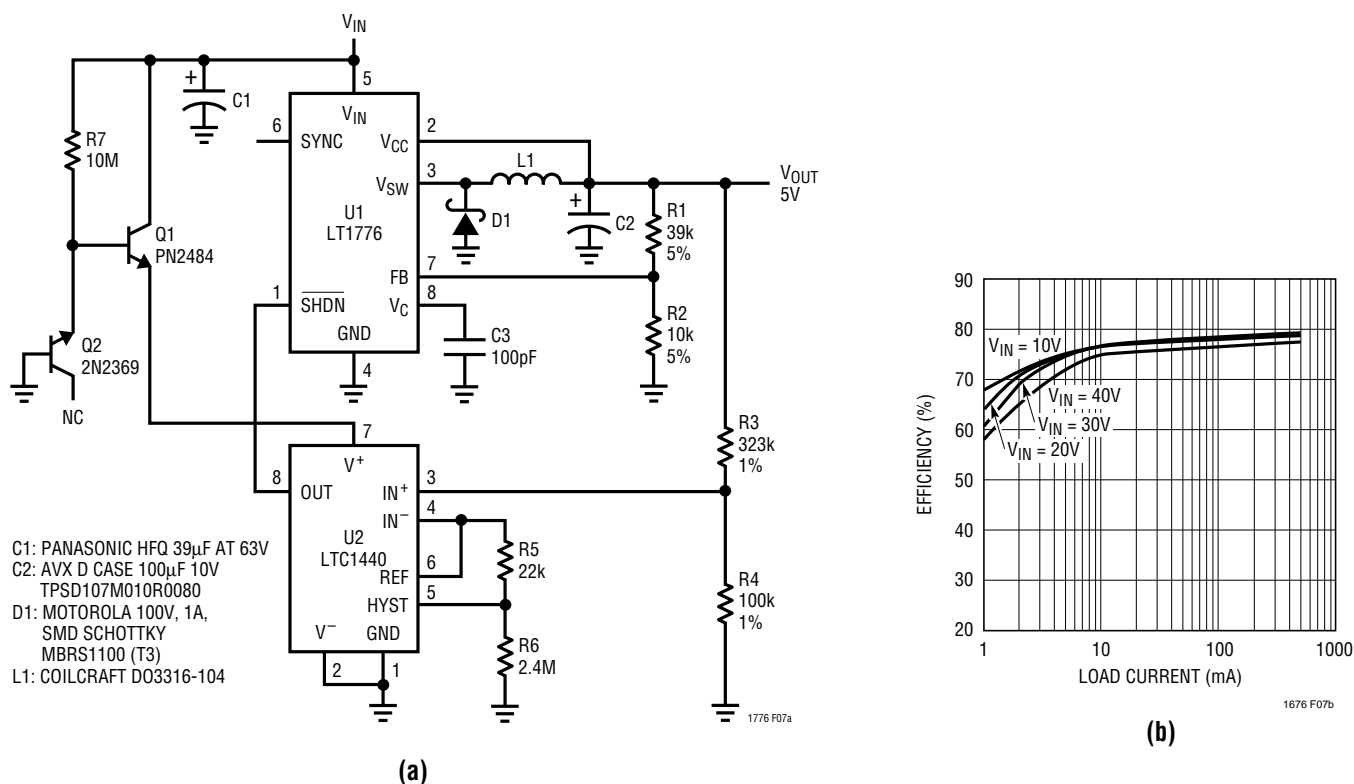
Figure 7. Burst Mode Operation Configuration for High Efficiency at Light Load
