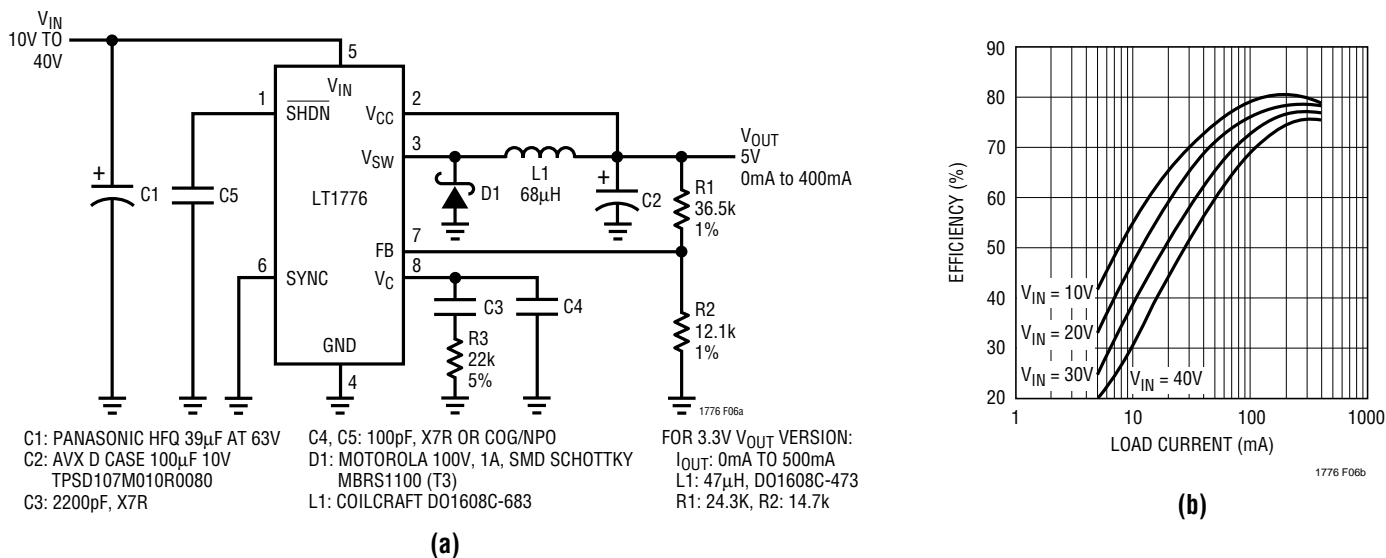
Figure 6. Minimum Inductor Size Application
