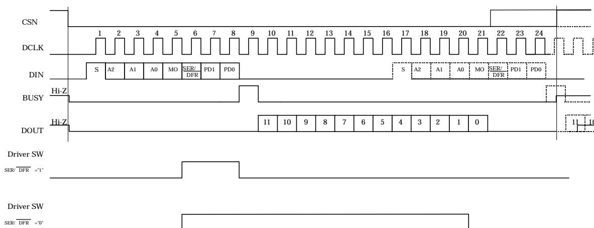
Figure 5 Serial Interface
