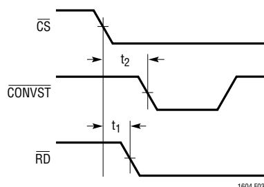
Figure 3. CS to CONVST Setup Timing
