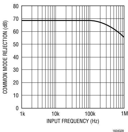
Figure 14. CMRR vs Input Frequency
