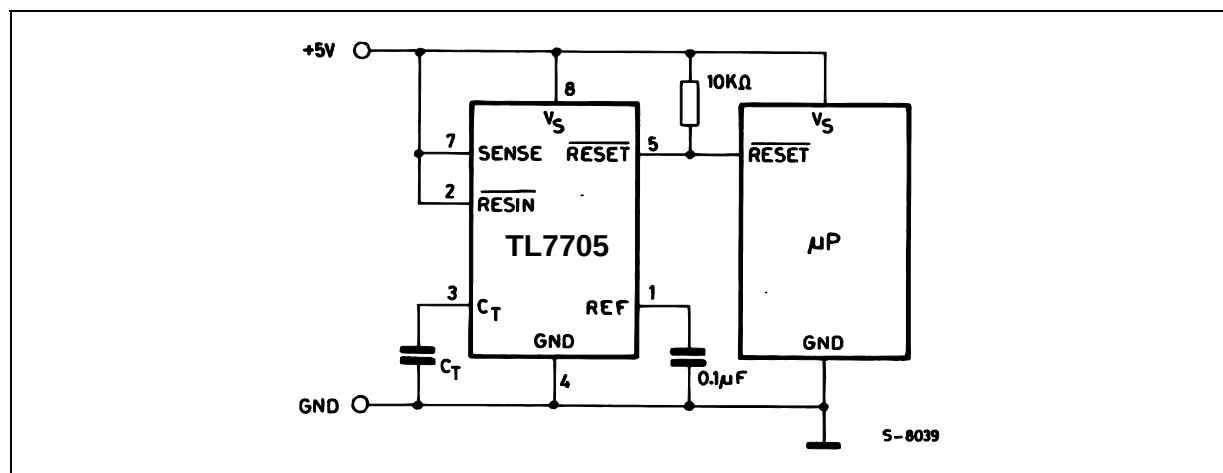
Figure 1 : Reset Controller for \mu\text{P}
