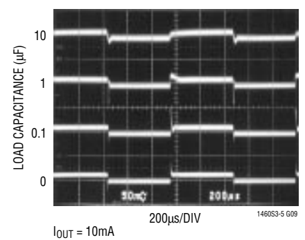
Transient Response
