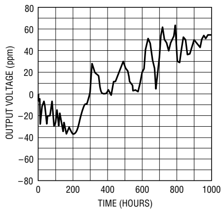
Typical Long-Term Drift
