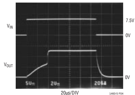
Figure 4. C_{IN} = 0
