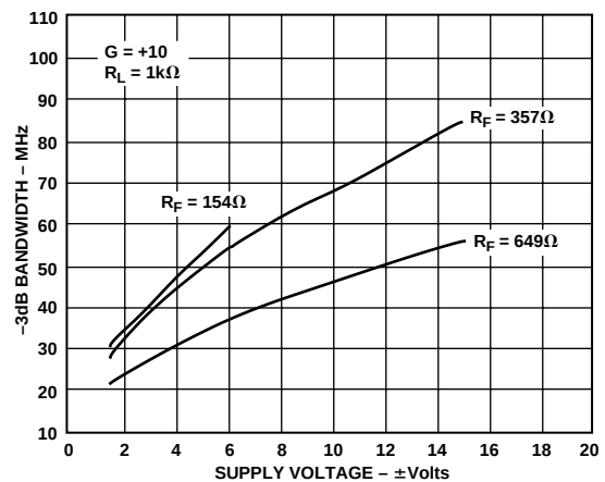
Figure 33. -3 dB Bandwidth vs. Supply Voltage, Gain = +10, R_L = 1 \text{ k}\Omega
