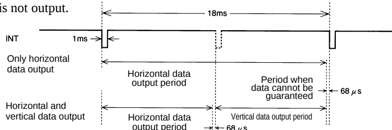
Figure 2 External Interface Basic Timing
