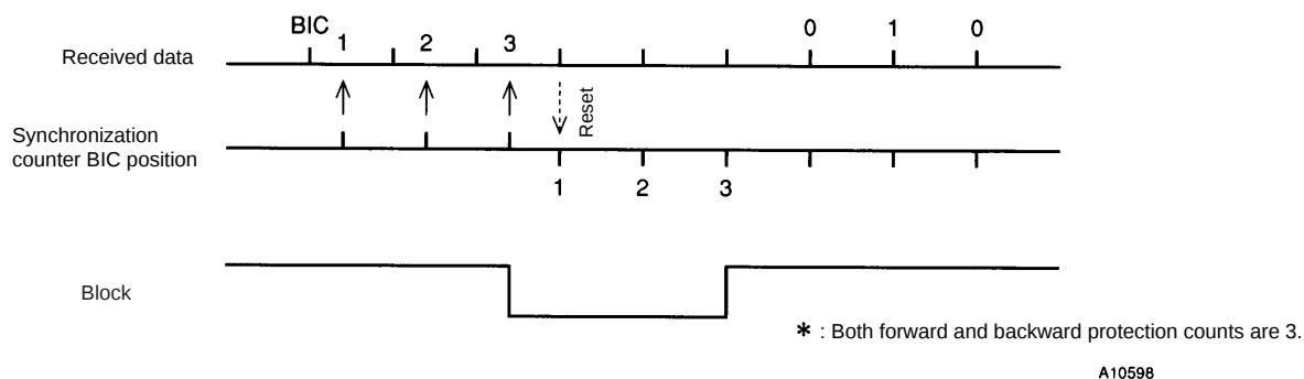
Figure 1 Block Synchronization Protection Operation (forward → backward → forward)
