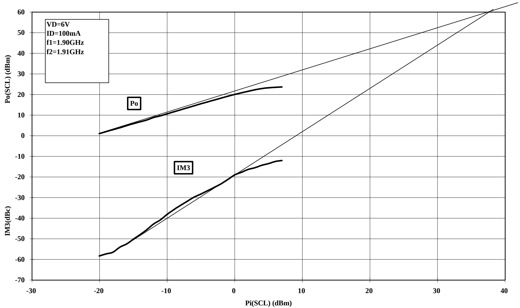
MGF0916A IM3, Po(SCL) vs. Pi(SCL)
