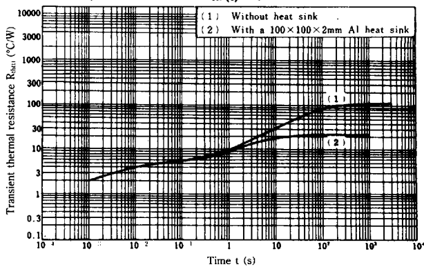
R_{th}(t) - t
