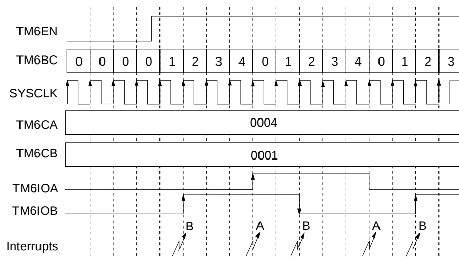
Figure 4-3-4 Two-phase PWM Timing
