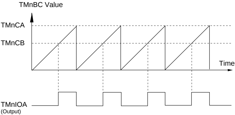
Figure 4-1-3 PWM Output Timing (Timer 6 and Timer 7)
