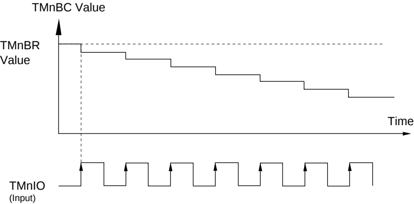
Figure 4-1-1 Event Counter Timing (Timer 0 to Timer 5)
