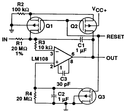
Figure 18. Low-Drift Integrator With Reset
