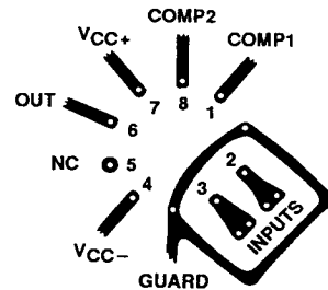
Figure 14. Input Guarding
