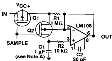
Figure 20. Inverting Amplifier With High Input Resistance
