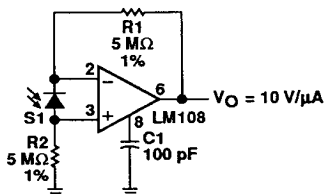
Figure 24. Amplifier for Photodiode Sensor
