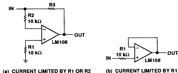
Figure 16. Input Protection
