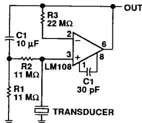
Figure 21. Amplifier for Piezoelectric Transducers
