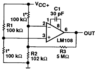
Figure 19. Amplifier for Bridge Transducers
