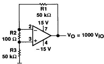
Figure 17. Test Circuit for Input Offset Voltage
