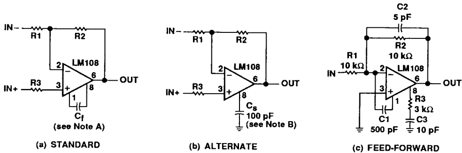
Figure 13. Frequency Compensation Circuits
