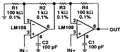
Figure 25. Differential-Input Instrumentation Amplifier
