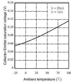
Collector-Emitter saturation voltage Vs. Ambient temperature
