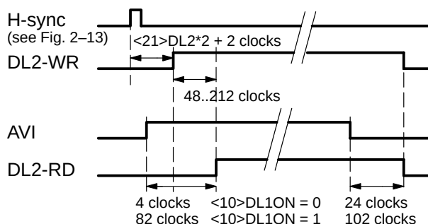
Fig. 2–14: DL2-setup (<17>PXSKWON = 1)
