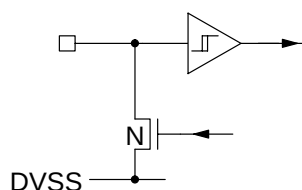
Fig. 3–6: Input pins 31 and 32
