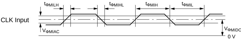
Fig. 3–14: Main clock input
