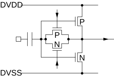
Fig. 3–9: Input pin 54
