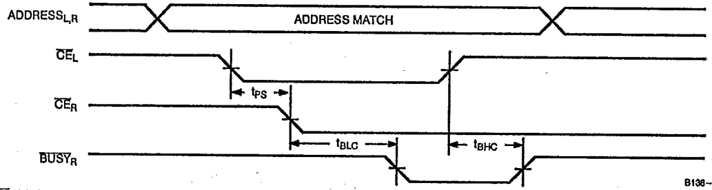
Busy Timing Diagram No. 1 (CE Arbitration) [30]
