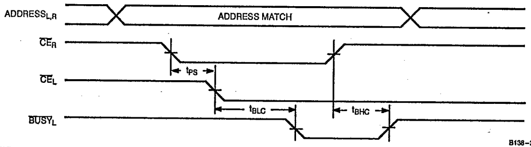
Busy Timing Diagram No. 2 (Address Arbitration) [30]
