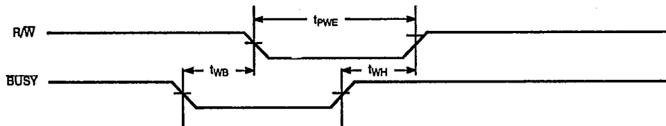
Write Timing with Busy Input ( M/\bar{S}=\text{LOW} )
