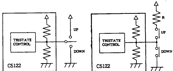
(Detent SW interface)
