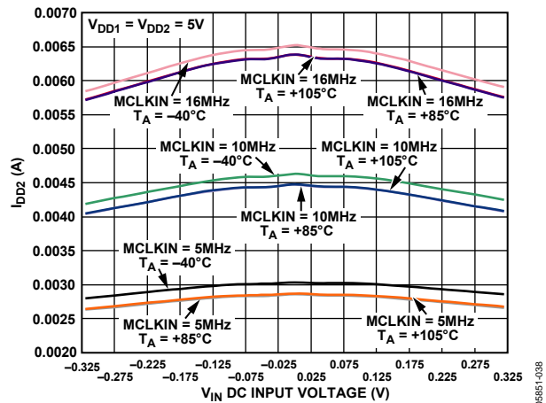
Figure 17. I DD2 vs. V IN at Various Temperatures
