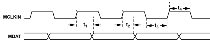
Figure 3. Data Timing
