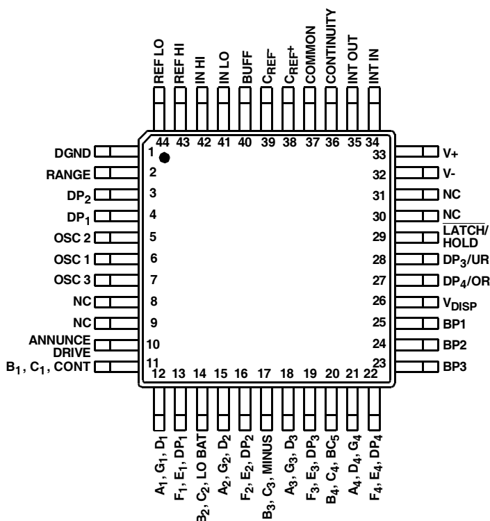
ICL7129 (MQFP) TOP VIEW
