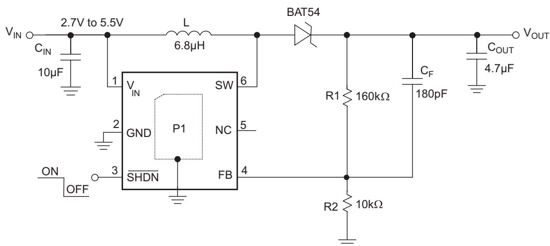
Figure 3. Test Circuit
