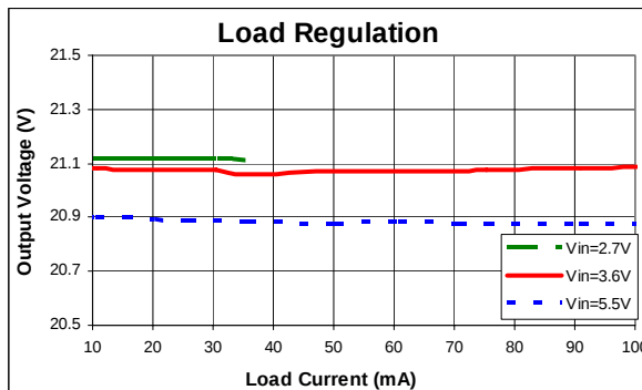
Figure 5. Load Regulation
