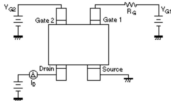
Test Circuit for Operating Items ( I_{D(on)} , |y_{fs}| , C_{iss} , C_{oss} , C_{rss} , NF, PG)
