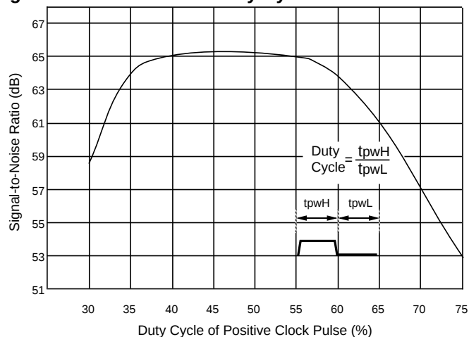
Figure 4 - SNR vs Clock Duty Cycle
