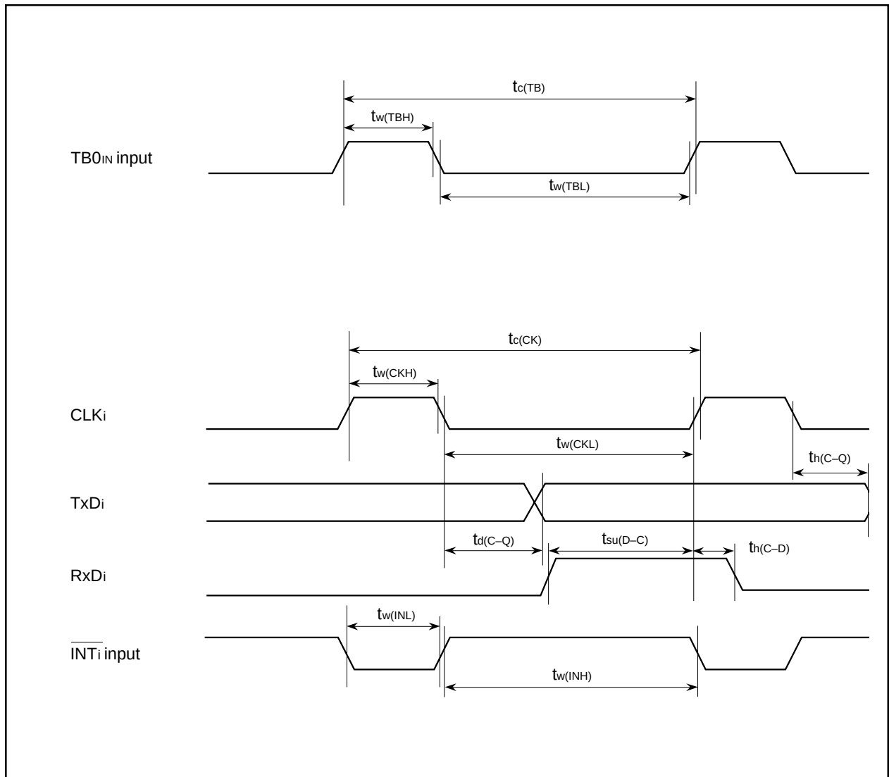
Figure 5.8.1 Timing diagram
