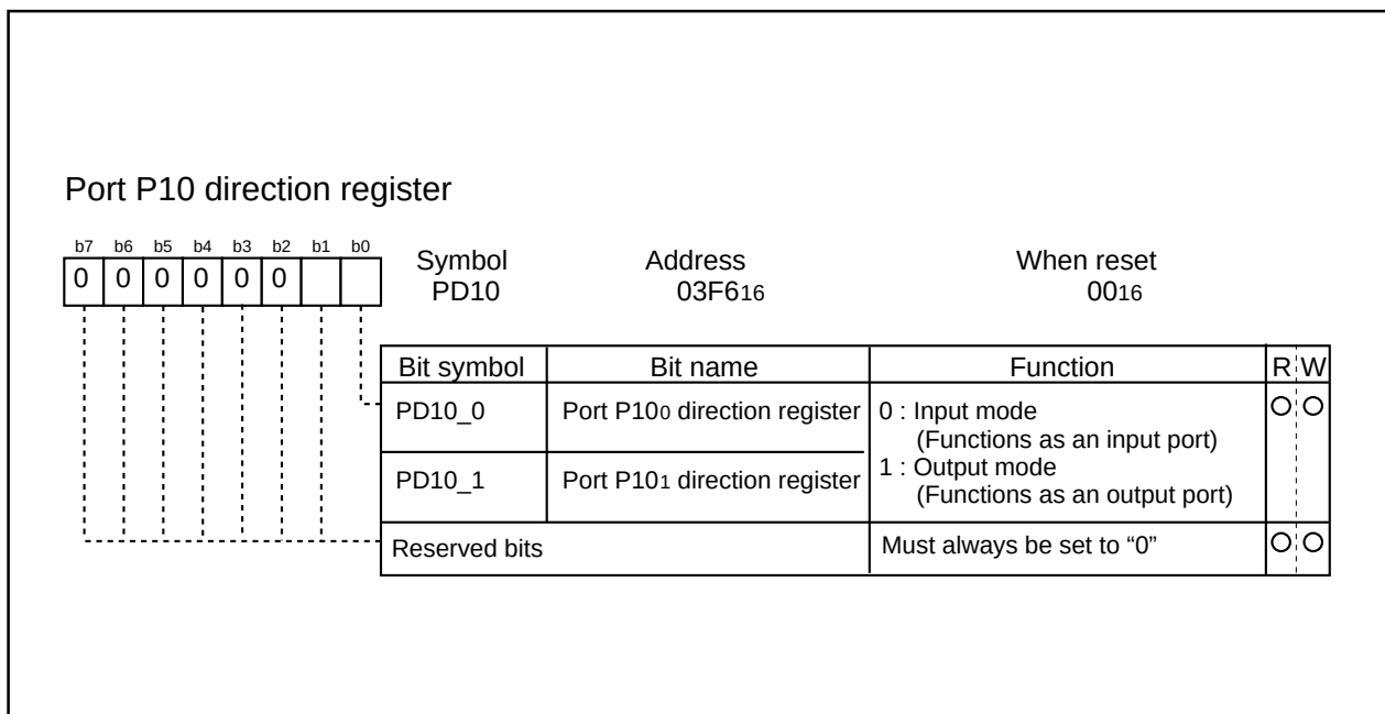
Figure 2.17.12 Port P10 direction register
