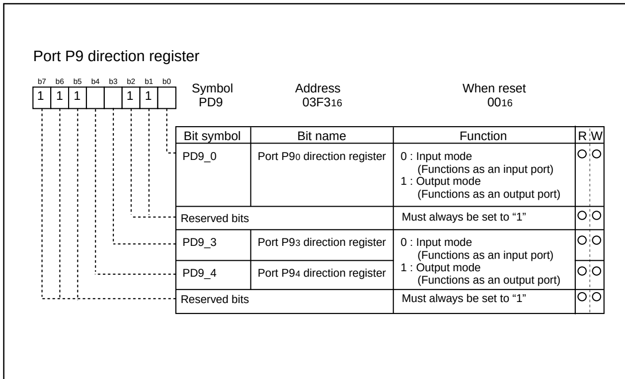
Figure 2.17.11 Port P9 direction register
