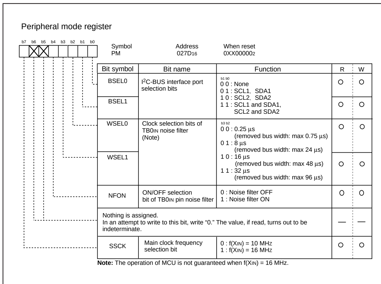
Figure 2.10.28 Peripheral mode register
