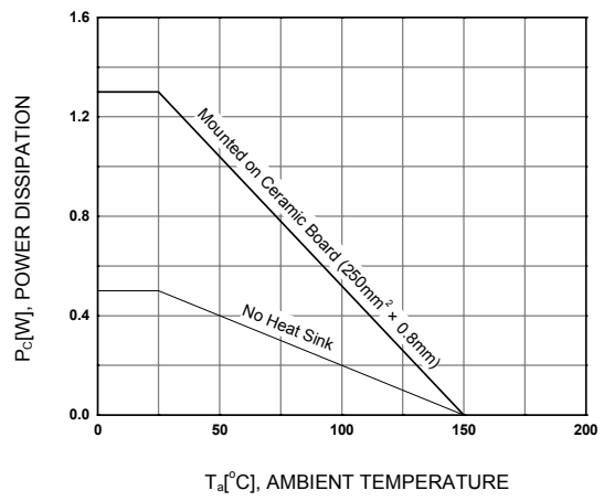
Figure 8. Power Derating
