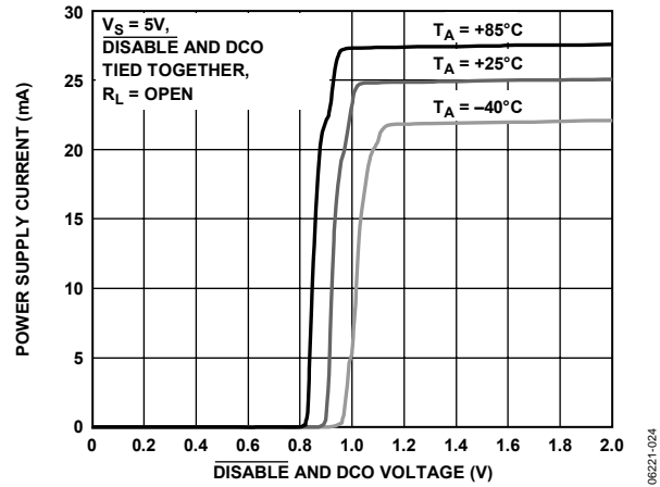
Figure 24. Supply Current vs. \overline{\text{DISABLE}}/\text{DCO} Voltage and Temperature
