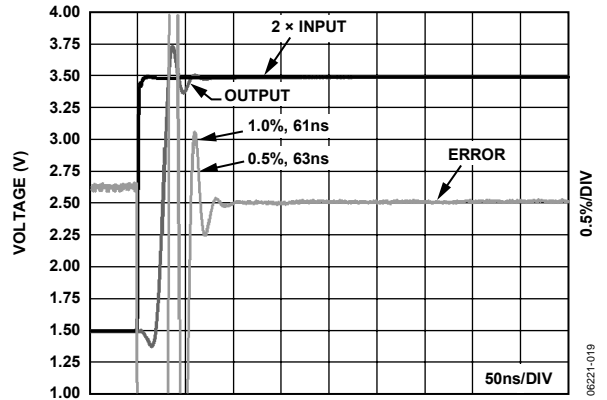
Figure 19. Settling Time
