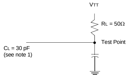
Load Circuit
