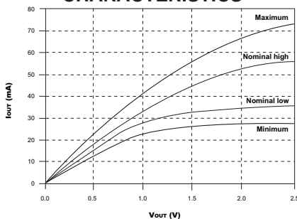
FIG. C REDUCED DRIVE PULL-DOWN CHARACTERISTICS
