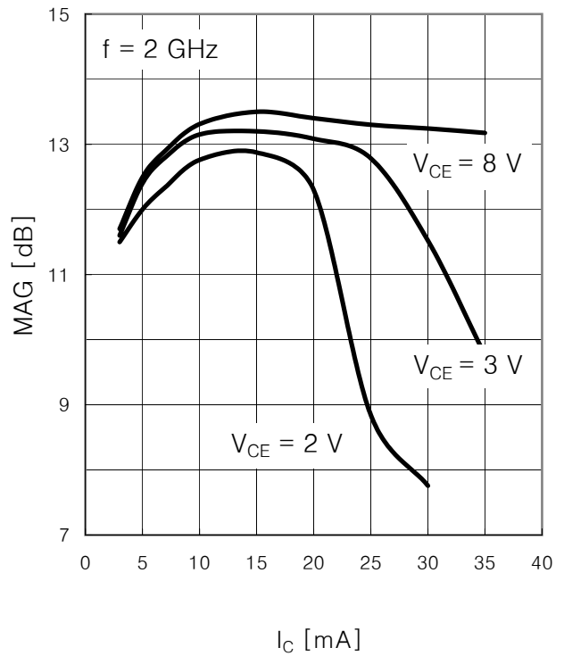
Maximum Available Gain, MAG vs. I C
