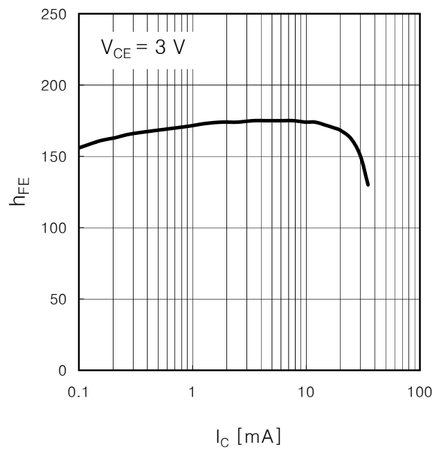
h_{FE} vs. I_C
