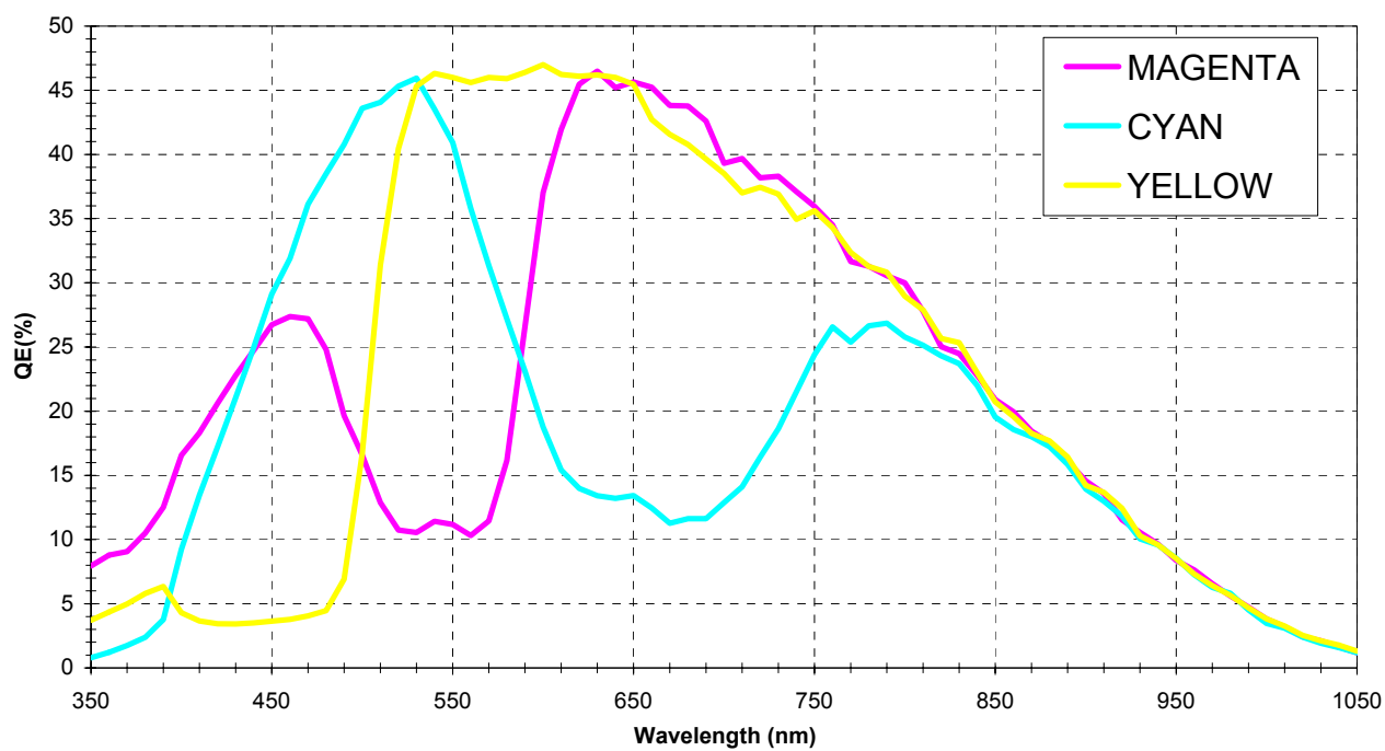
Figure 16: KAC-1310 Typical Bayer CMY Spectral Response
