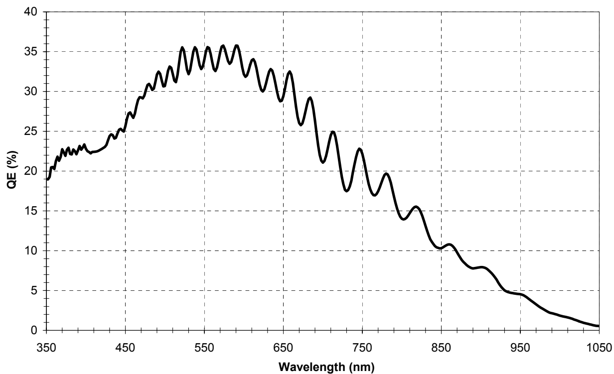
Figure 14: KAC-1310 Typical Monochrome Spectral Response
