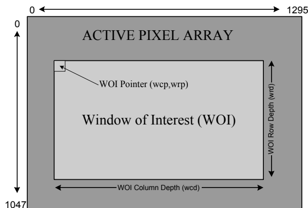
Figure 7: WOI Definition
