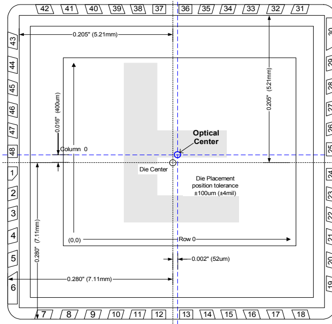
Figure 1. Pinout Diagram
