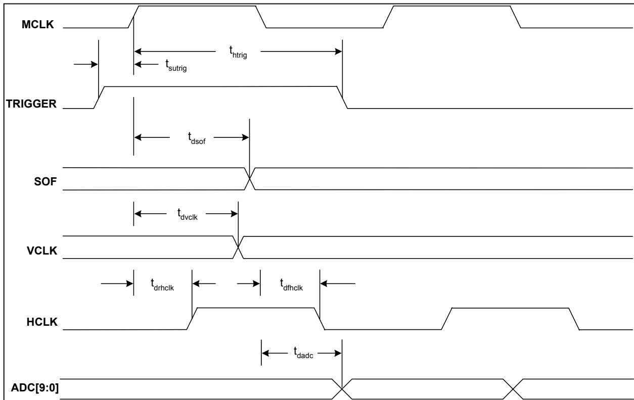
Figure 23: Pixel Data Bus Timing Diagram
