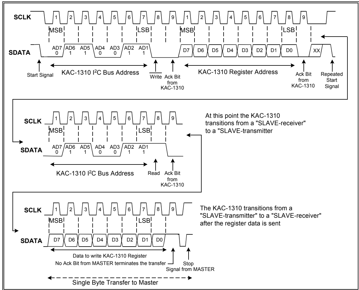
Figure 26: I²C Bus READ Cycle
