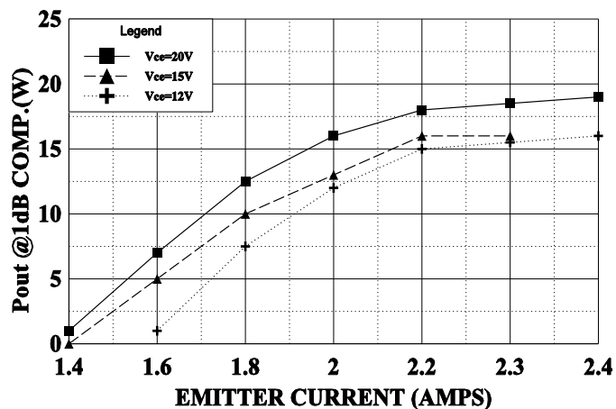
1dB COMPRESSION POINT vs EMITTER CUR.
