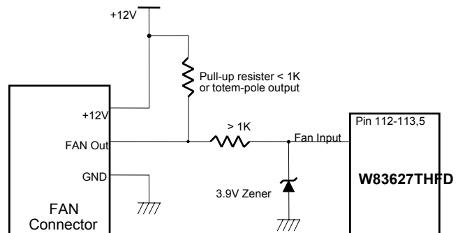
Figure 5-7. Fan with Tach Pull-Up to +12V, or Totem-Pole Output and Zener Clamp
