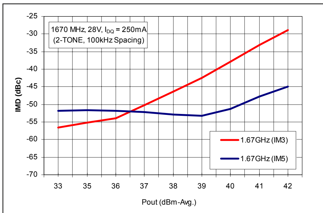
Graph 2. Two Tone: Intermodulation Distortion vs. Output Power
