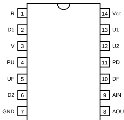
Figure 2. Pin Diagram
