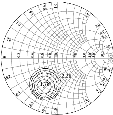
Ids=400mA
