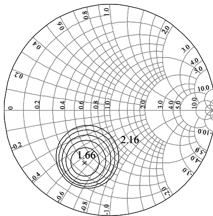
Ids=350mA
