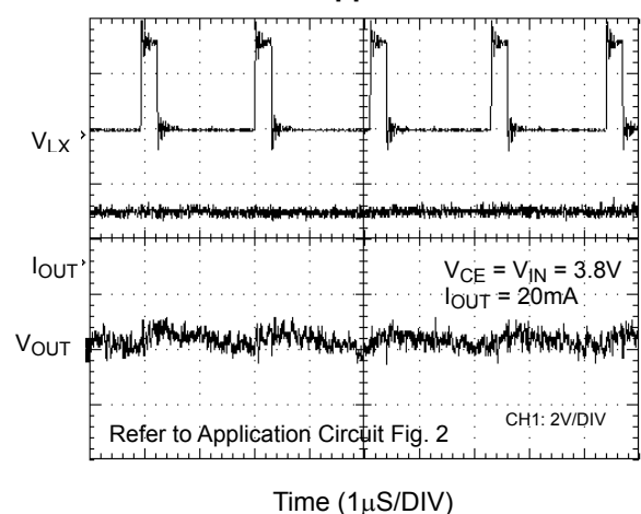
LX vs. Ripple Waveform
