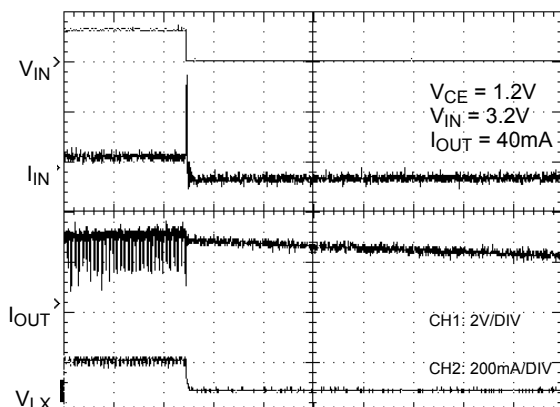
Shutdown Waveform
