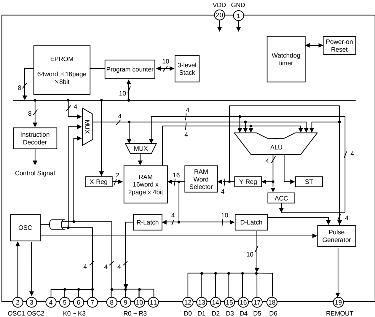
Fig 2-1 Block Diagram
