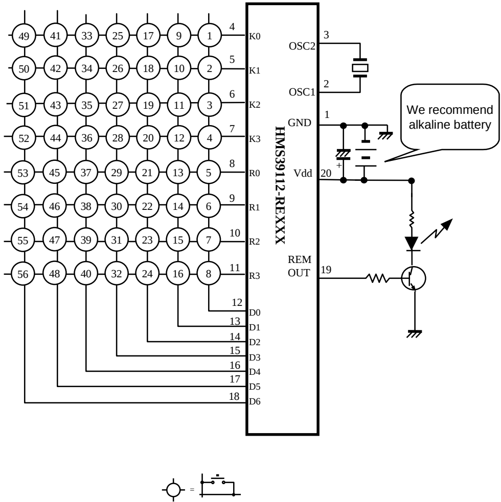
HMS39112 Circuit Diagram
