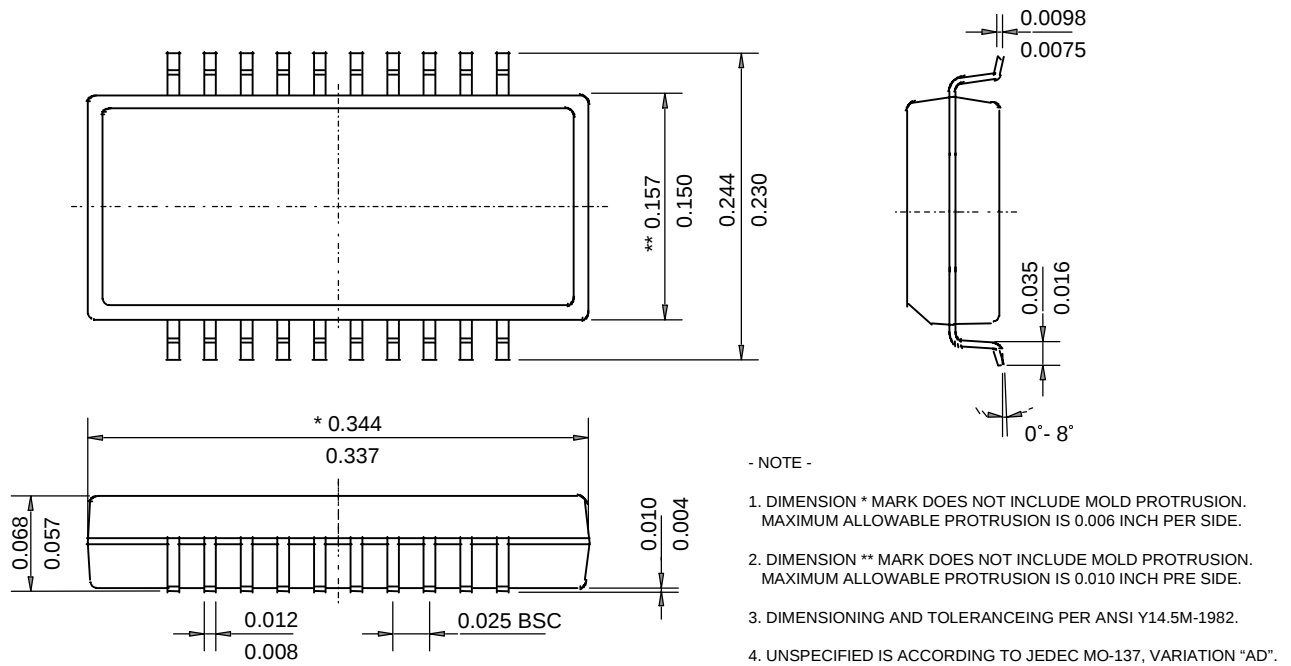
Fig 1-5. 20SSOP (150MIL) Pin Dimension (UNIT : inch)
