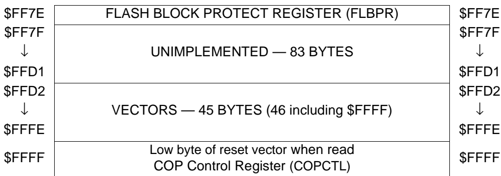
Figure 2-1. Memory Map
