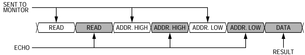
Figure 10-4. Read Transaction
