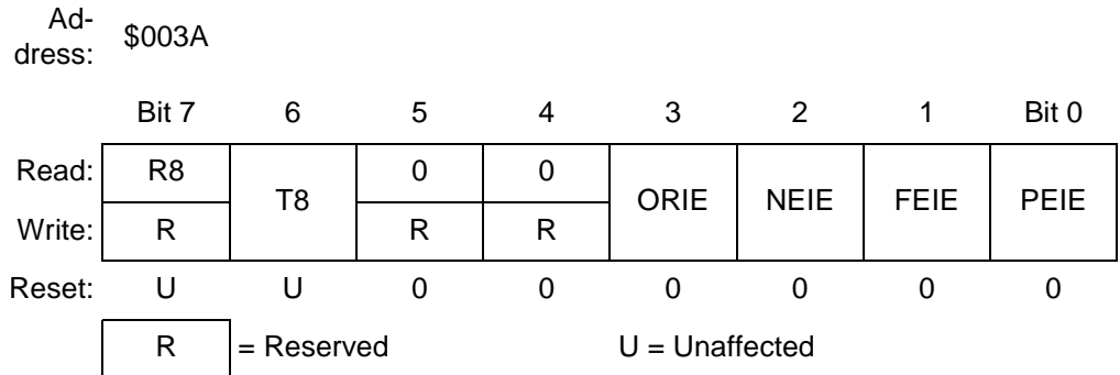
Figure 13-9. SCI Control Register 3 (SCC3)
