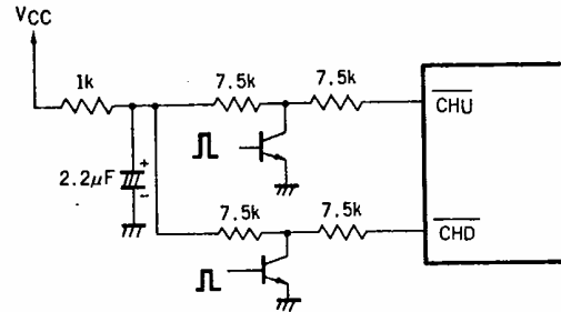
(c) Remote Control Use (Short Pulse Width)
