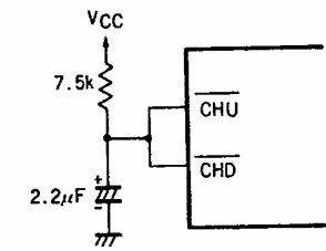
(a) Only Channel Selection Use
