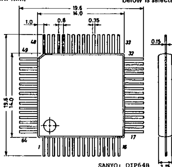
Case Outline 3026B-Q64B1C (unit: mm)
