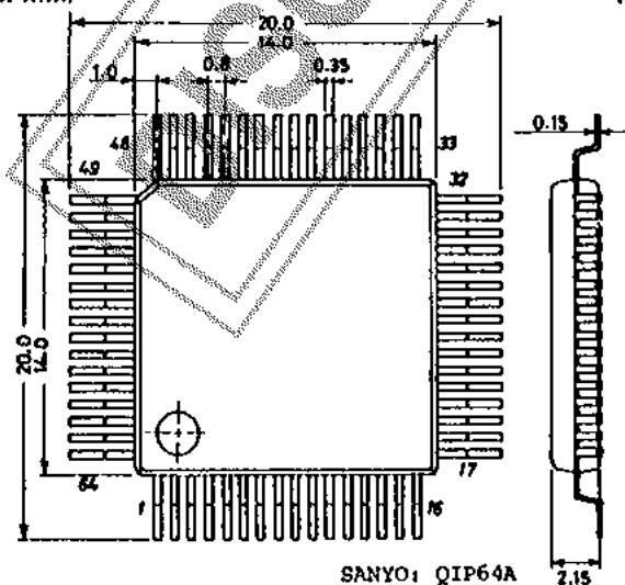
Case Outline 3057-Q64A1C (unit: mm)
