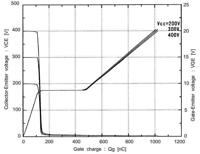
Dynamic input characteristics Tj=25°C
