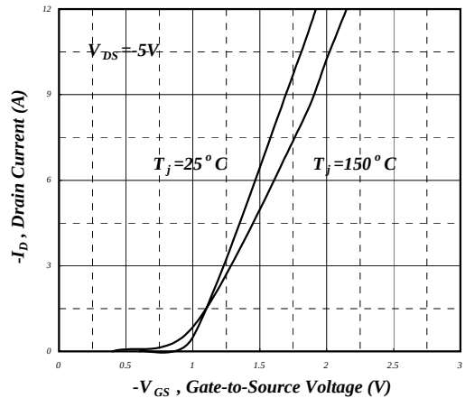
Fig 11. Transfer Characteristics
