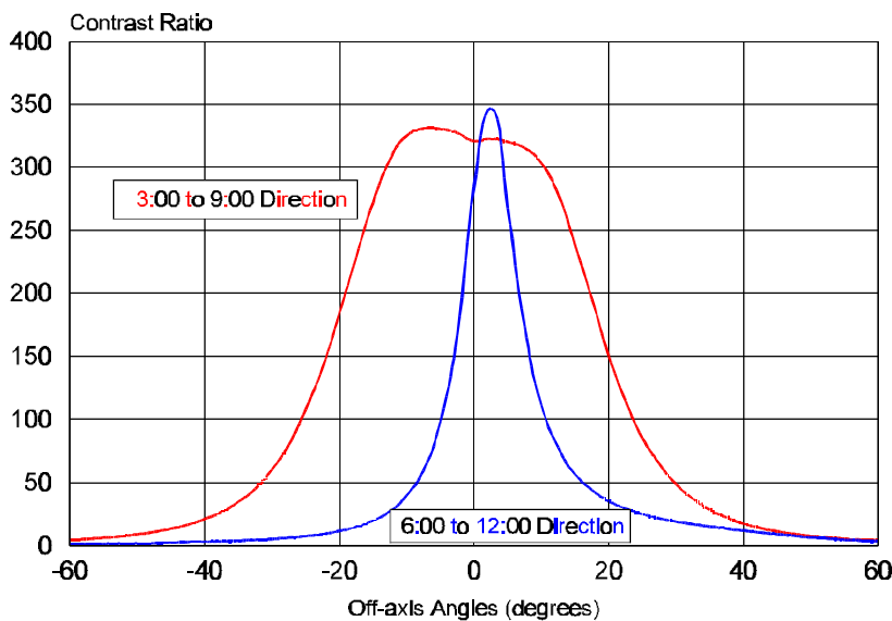
LM130A-12C318 LCD Contrast Ratio Angular Distribution
