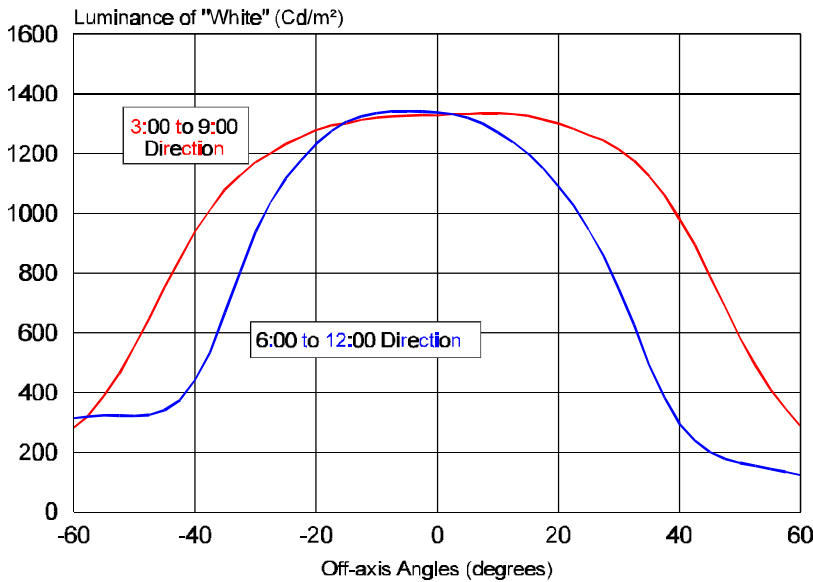
LM130A-12C318 LCD Screen Brightness Angular Distribution
