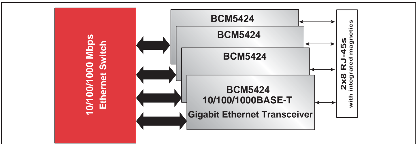
BCM5424 System Diagram
