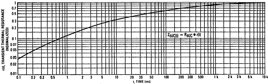
FIGURE 7 - THERMAL RESPONSE
