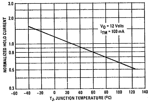
FIGURE 10 - HOLDING CURRENT
