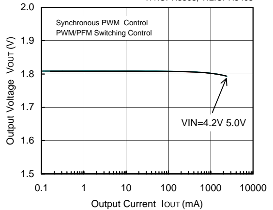
FOSC=180kHz, V OUT =1.8V
