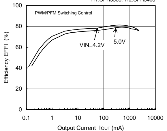
FOSC=180kHz, V OUT =1.8V
