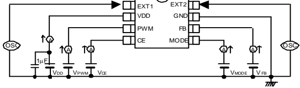
Circuit 4
