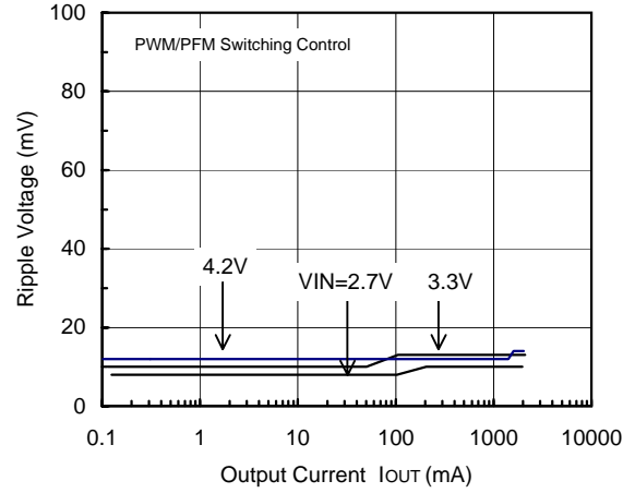
FOSC=300kHz, V OUT =1.2V
