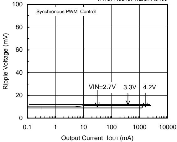
FOSC=300kHz, V OUT =1.8V
