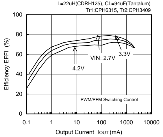
FOSC=300kHz, V OUT =1.2V
