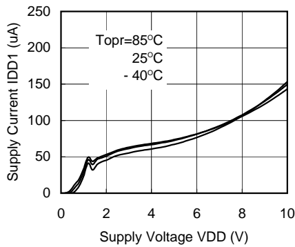
(7) Standby Current vs Supply Voltage
