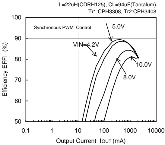
FOSC=300kHz, V OUT =1.2V
