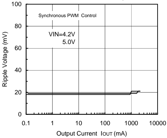
FOSC=180kHz, V OUT =1.8V
