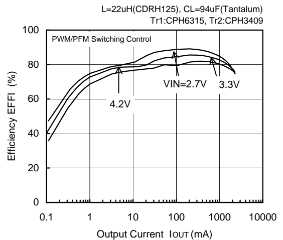
FOSC=300kHz, V OUT =1.8V
