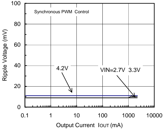
FOSC=300kHz, V OUT =1.2V
