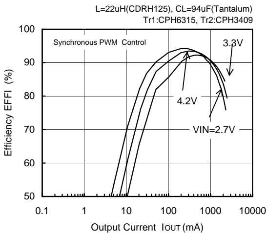
FOSC=300kHz, V OUT =1.8V
