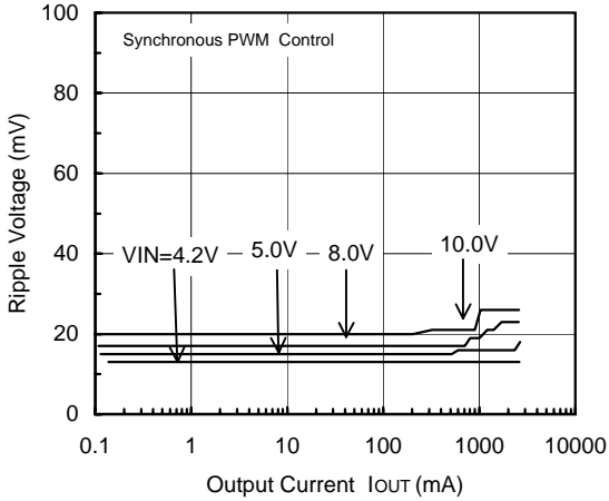
FOSC=300kHz, V OUT =3.3V
