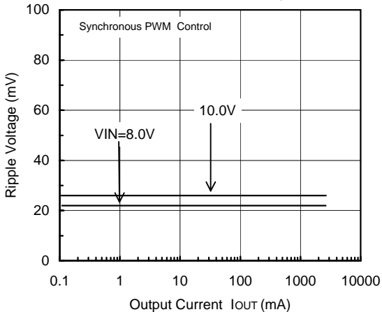
FOSC=300kHz, V OUT =5.0V
