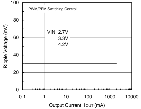
FOSC=300kHz, V OUT =5.0V
