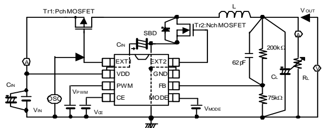
Circuit 4
