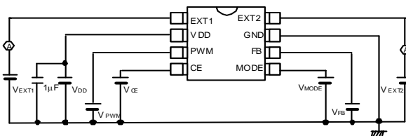
Circuit 5
