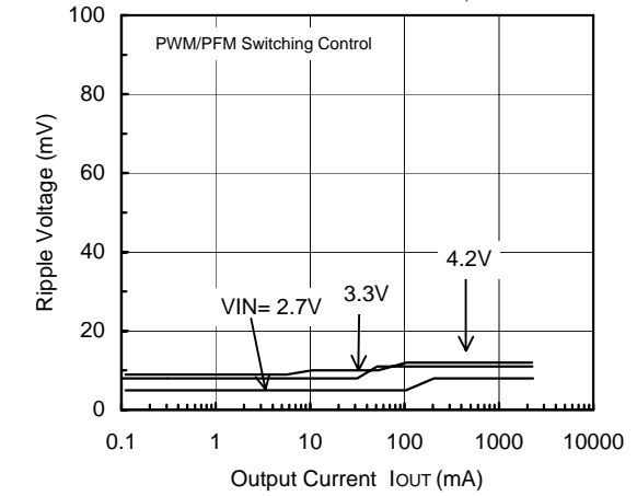
FOSC=300kHz, V OUT =1.8V
