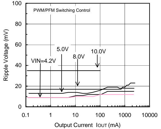
FOSC=300kHz, V OUT =3.3V
