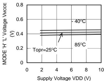
(12) MODE 'H' 'L' Voltage vs. Supply Voltage
