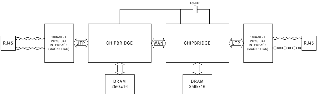
Figure 13. Local Bridge
