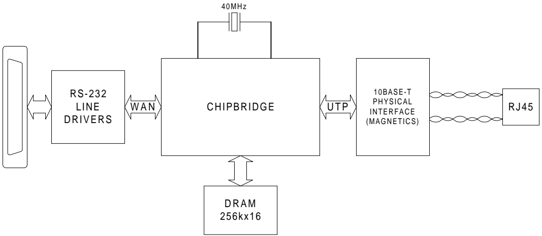
Figure 12. Remote Bridge
