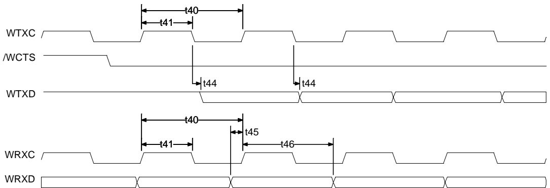
Figure 11. WAN Synchronous Mode Timing
