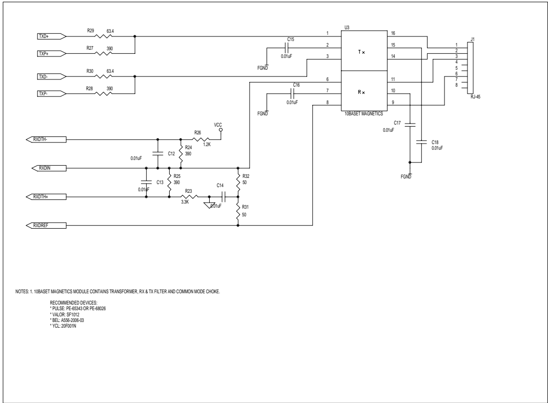
Figure 16. UTP Interface
