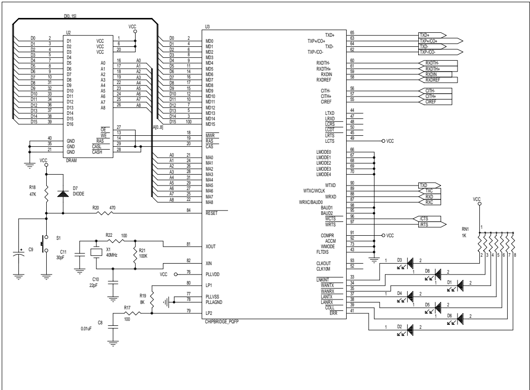
Figure 15. ChipBridge Connection
