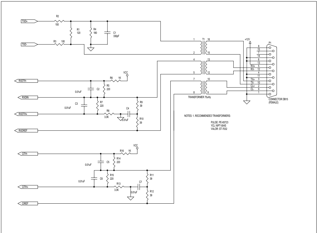
Figure 17. AUI-DTE Interface
