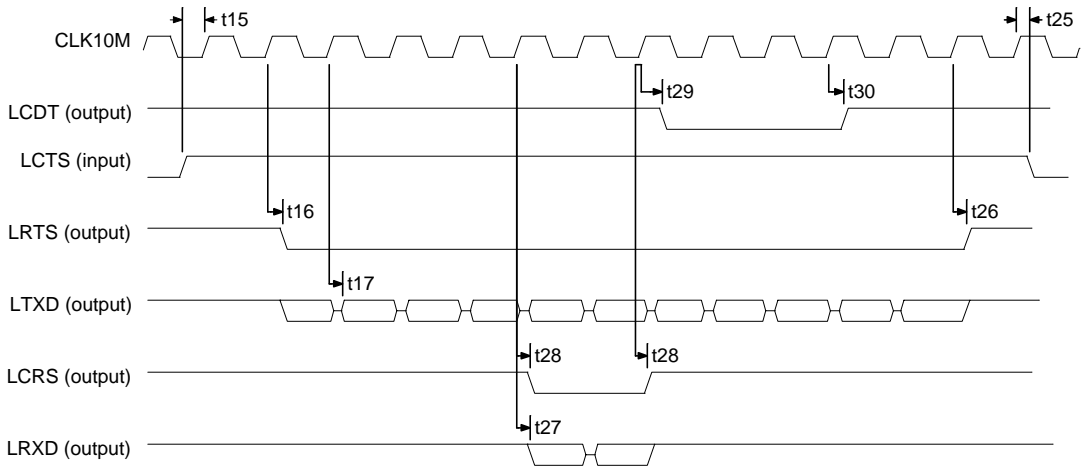
Figure 7. NRZ Transmit and Receive Timing (outputs)
