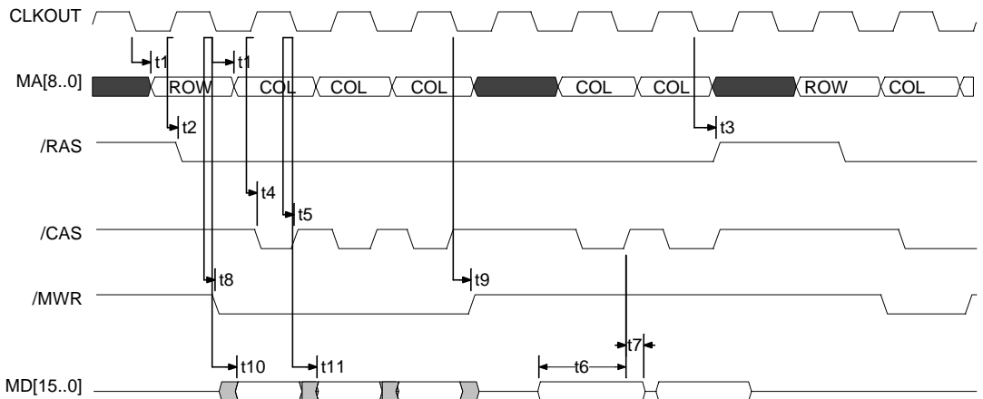
Figure 4. Burst-Mode DRAM Read and Write Timing
