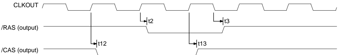
Figure 5. DRAM CAS-Before-RAS Refresh Timing
