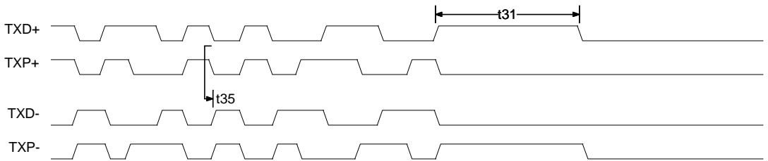
Figure 10. UTP Mode Timing
