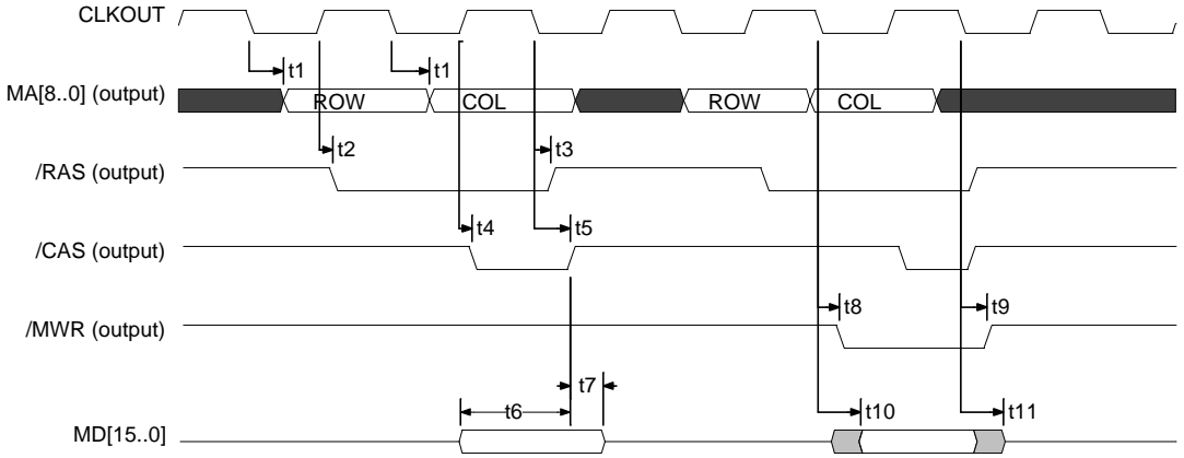
Figure 3. Single Cycle DRAM Read and Write Timing
