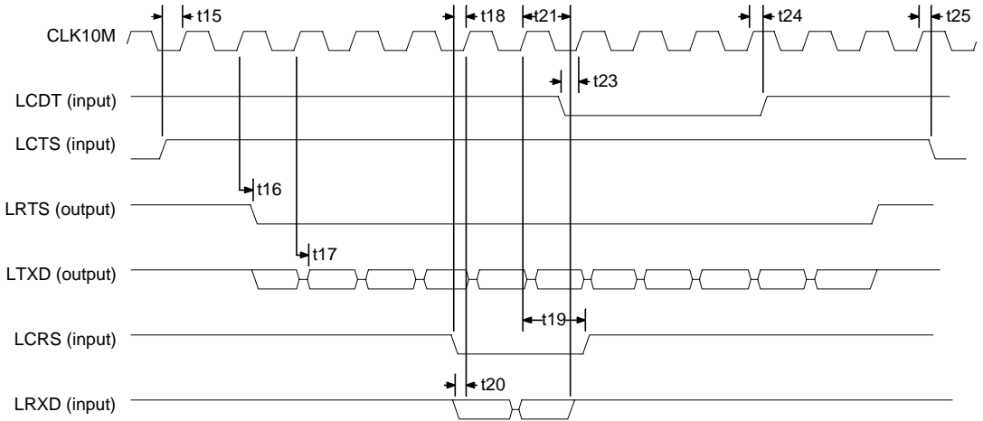
Figure 6. NRZ (Mode 1) Transmit and Receive Timing (inputs)
