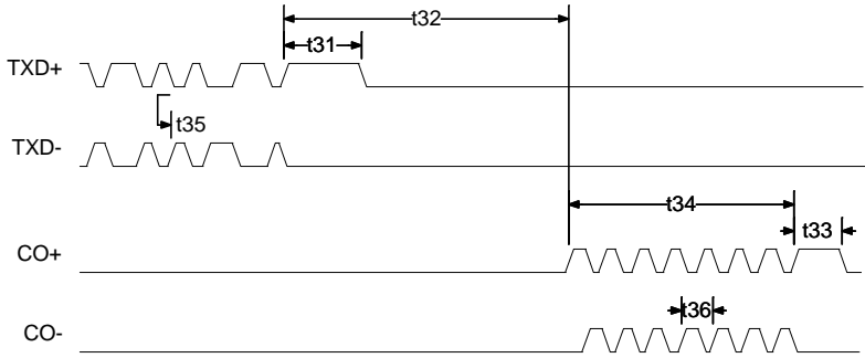
Figure 9. AUI-DCE Mode Timing
