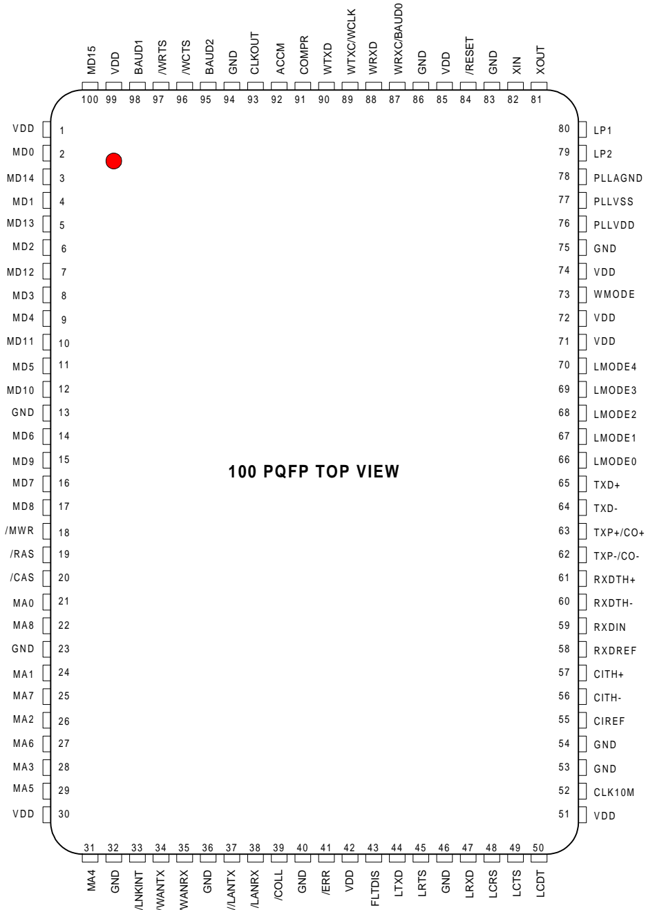
Figure 2. Connection Diagram
