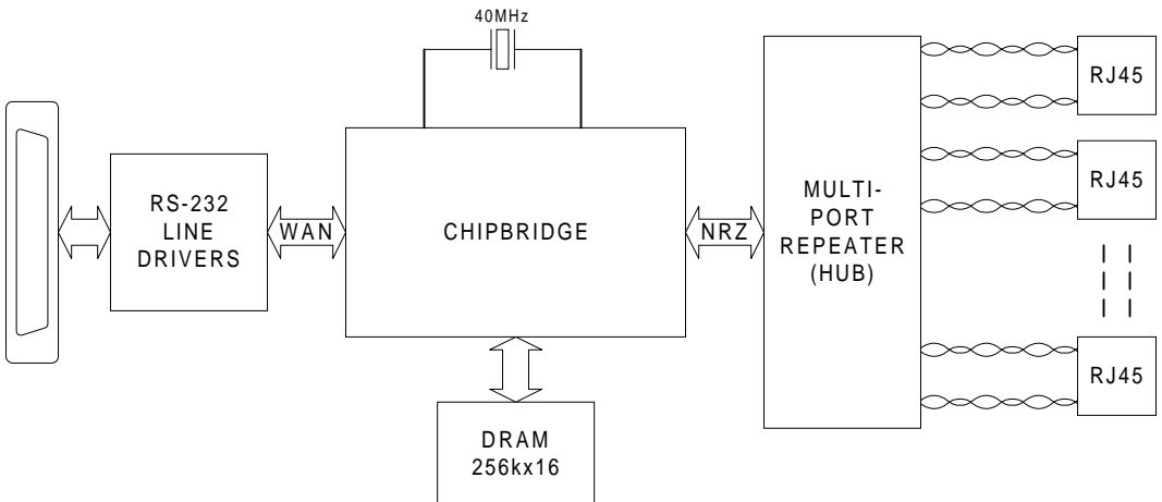
Figure 14. Connection to HUB
