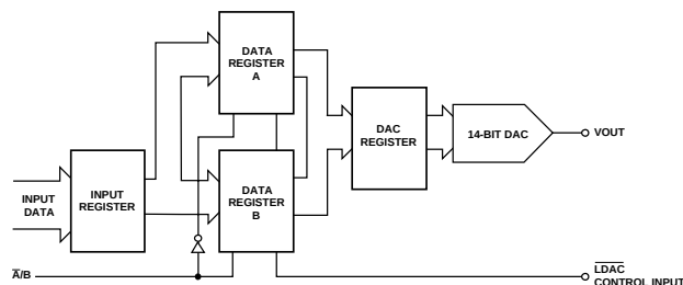
Figure 43. Toggle Mode Function
