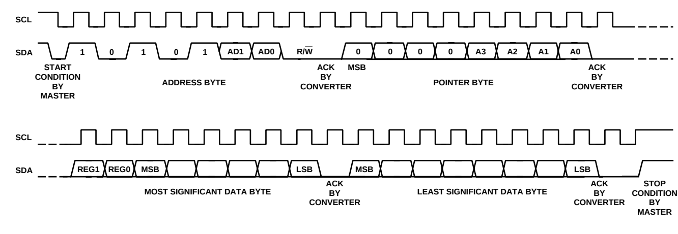
Figure 33. The 4-Byte Mode I 2 C Write Operation
