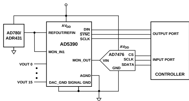
Figure 42. Typical Channel Monitoring Circuit
