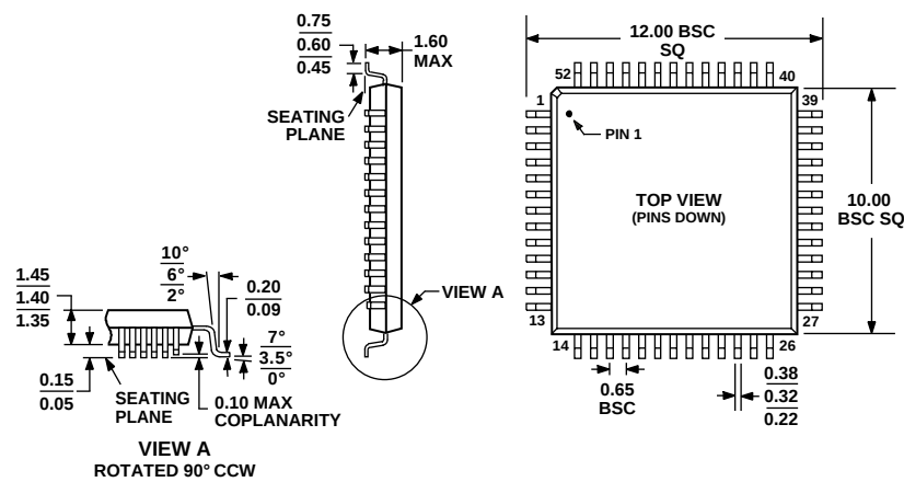
COMPLIANT TO JEDEC STANDARDS MS-026BCC Figure 48. 52-Lead Low Profile Quad Flat Package [LQFP] (ST-52) (Dimensions shown in millimeters)
