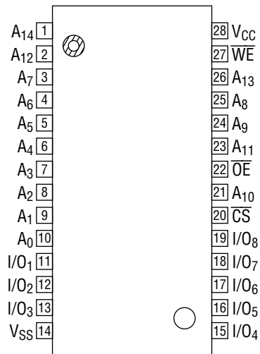
28-Pin Plastic SOP
